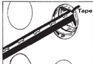
Step 5: Move the MaxBag into the duct making sure the body of the MaxBag maintains its cylindrical shape and the outer side of the bag is completely within the duct opening. Adjust the sealing bag to the inner shape of the tube. In the case of two or more cables occupying the conduit, wrap the bag around all cables. Do not allow the bag to create a separation between the cables.
